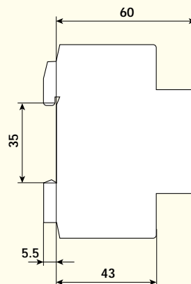
Side Elevation
